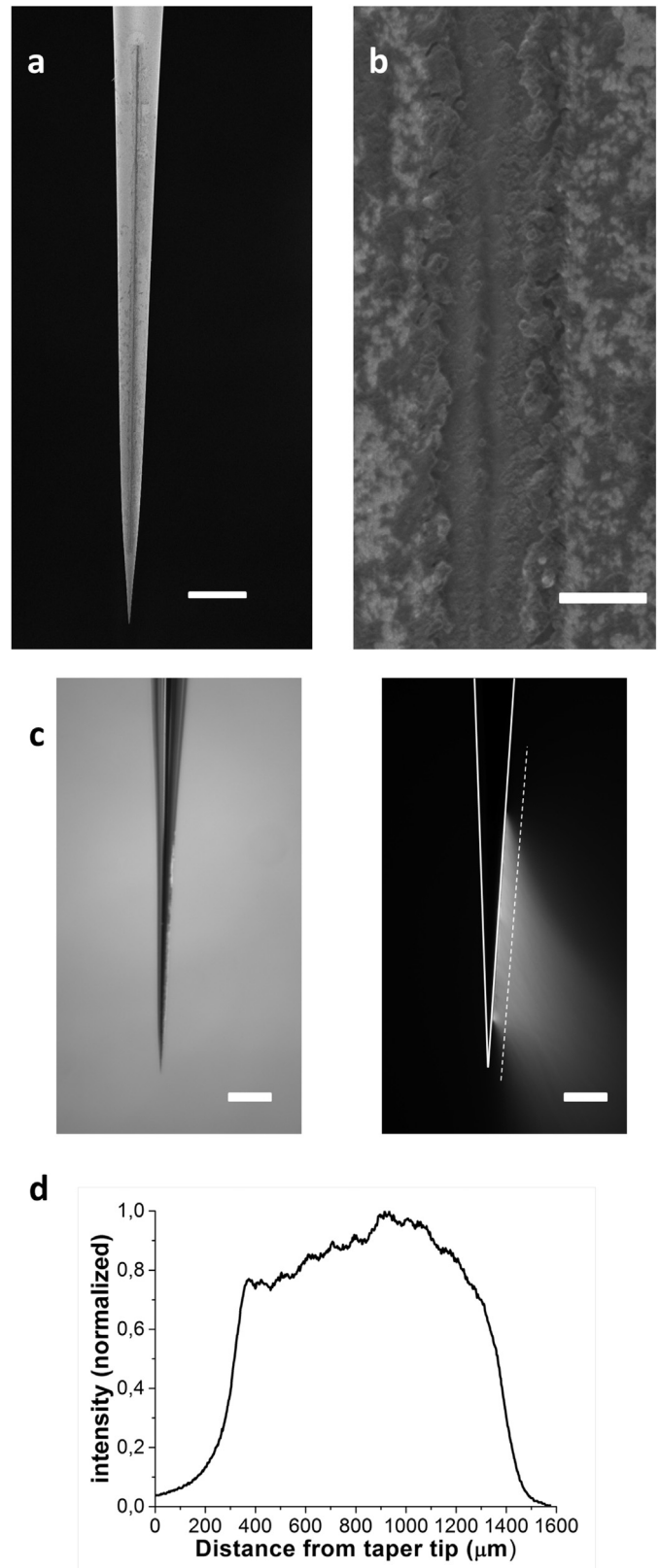
Fig. 7. (a, b) SEM micrographs of the single-slot device at two different magnifications. Scale bar represents 300 \mu\text{m} in panel a and 4 \mu\text{m} in panel b. (c) Bright-field (left) and emission (right) images of the single-slot device immersed in a drop of fluorescein. The white continuous lines outline the taper edges. Scale bars represent 200 \mu\text{m} . (d) Intensity profile collected along the white dashed line displayed in panel c.
