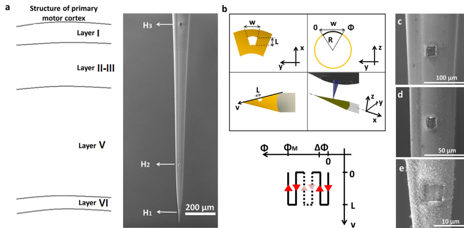
Fig. 3. (a) Schematic representation of primary motor cortex of the mouse brain (left) and SEM micrograph of the three-window device (right). The three windows are labeled as H1, H2, and H3. (b) Different views of the patterned geometry and definition of axes and sizes (Top). (Bottom) Schematic representation of the implemented raster scan to obtain a L \times W window along the v and \Phi . (c–e) SEM micrographs of H 3 , H 2 and H 1 , respectively.
