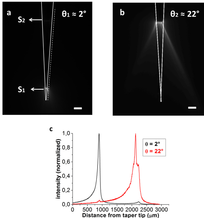
Fig. 6. (a, b) Emission from the two rings realized along the taper for two different input angles ( \theta_1 = 2^\circ , \theta_2 = 22^\circ in panel a and b, respectively). Scale bars represent 100 \mu\text{m} . The white continuous lines outline the taper edges. (c) Intensity profiles collected along the white dashed line displayed in panel a.
