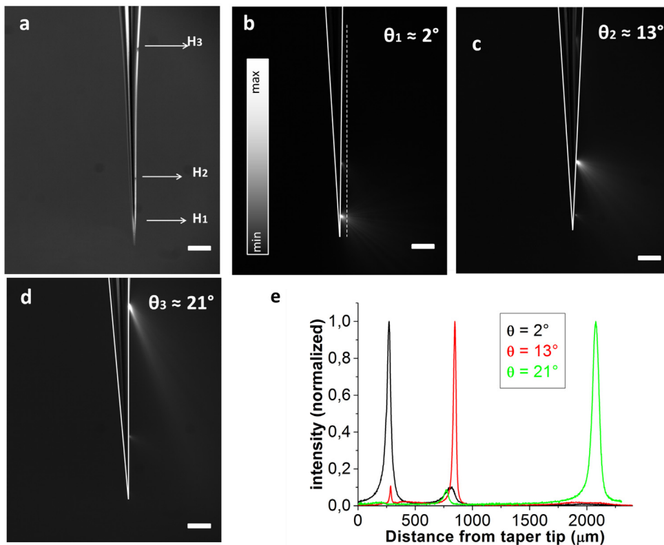
Fig. 4. (a) Bright-field image of the three-window device. Scale bar represents 200 \mu\text{m} . (b, c, d) Fluorescence images of the taper emission by setting three different input-coupling angles ( \theta_1 = 2^\circ , \theta_2 = 13^\circ , \theta_3 = 21^\circ in panel b, c, and d, respectively). The white continuous lines represent the taper edges. The white dashed line represents the region over which the light intensity profiles in panel e were acquired. Scale bars represent 200 \mu\text{m} . (e) Intensity profiles collected along the white dashed line displayed in panel c. Black, red and green curves represent the emission profiles from \theta = 2^\circ , \theta = 13^\circ and \theta = 21^\circ , respectively. (For interpretation of the references to colour in this figure legend, the reader is referred to the web version of this article.)
