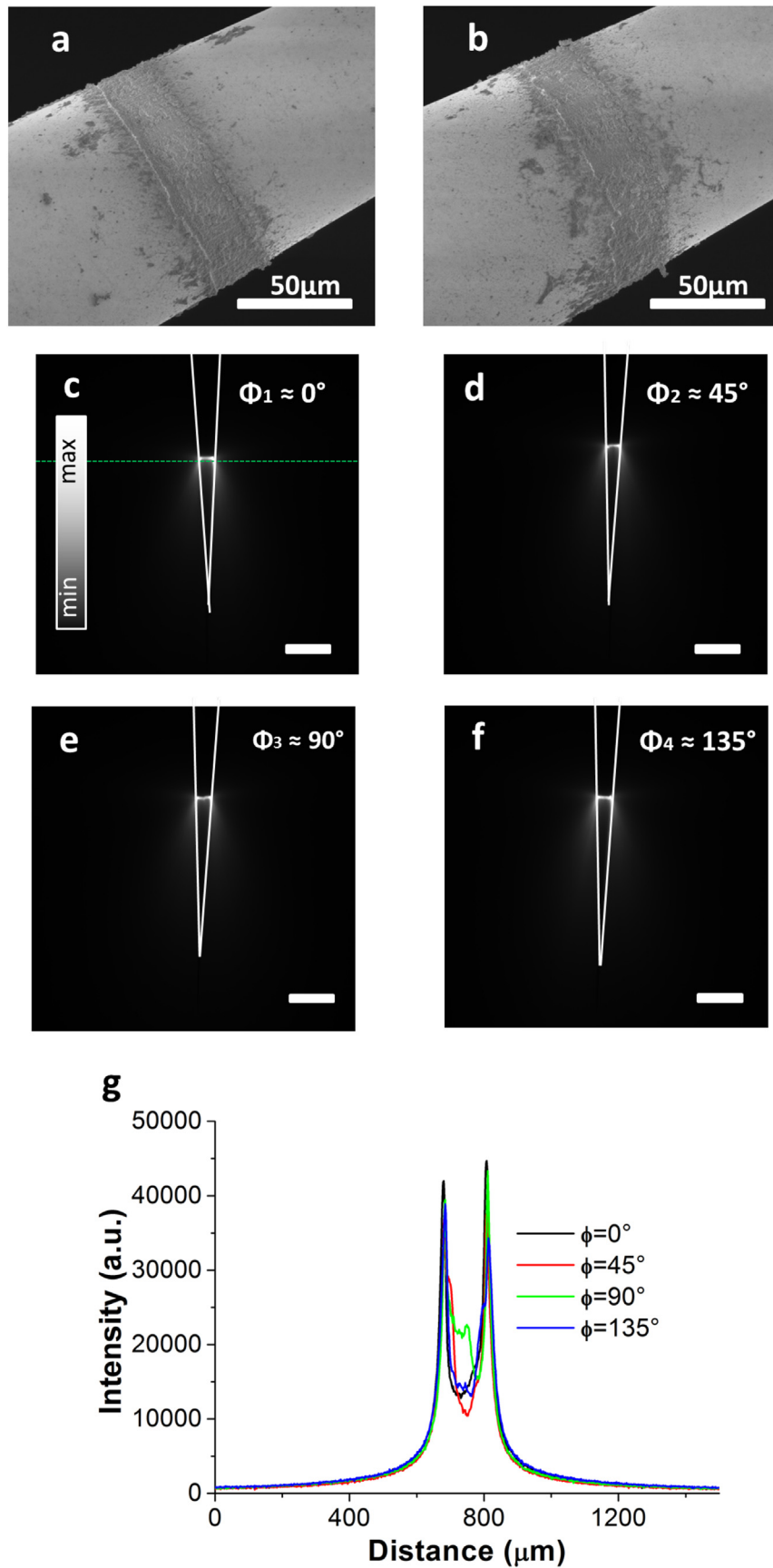
Fig. 5. (a, b) SEM images of the pattern ring-shaped window. The two images show two opposite sides of the taper (e.g. \phi = 0 and \phi = 180^\circ ). (c, d, e, f) Fluorescence images of the taper emission from four different sides of the taper ( \phi_1 = 0^\circ , \phi_2 = 45^\circ , \phi_3 = 90^\circ and \phi_4 = 135^\circ ). Scale bars represent 200 μm. Taper edges are highlighted by the white continuous lines. (g) Overlay of the Intensity profiles collected along normal direction to the fiber optical axis (green dashed line in panel c). (For interpretation of the references to colour in this figure legend, the reader is referred to the web version of this article.)
