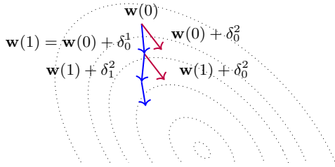
Fig. 2. Gradient descent in \mathbf{w} space. \delta_i^j = -\eta \nabla L(\mathbf{w}(i), \mathbf{x}_j) represents the gradient calculated on the weights updated up to step i , based on sample (or mini-batch) \mathbf{x}_j . Therefore, the red update based on \delta_0^2 is outdated with respect to \mathbf{w}(1) , but its impact is not necessarily detrimental to the training. The target function is L: \mathbb{R}^m \rightarrow \mathbb{R} .
